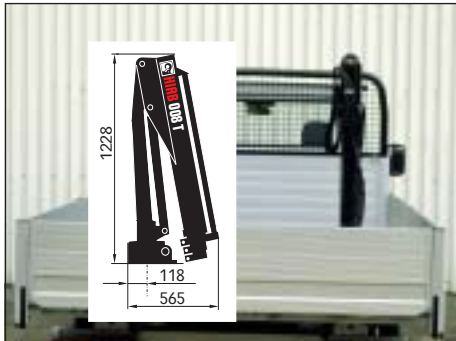
The HIAB 008 T requires the minimum of platform space, and it is so low that it goes in under most pick-up-truck covers.
