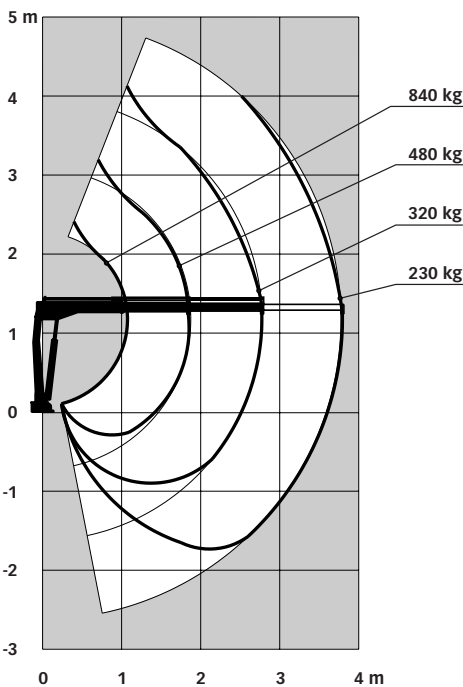
The HIAB 008 T requires the minimum of platform space, and it is so low that it goes in under most pick-up-truck covers.
